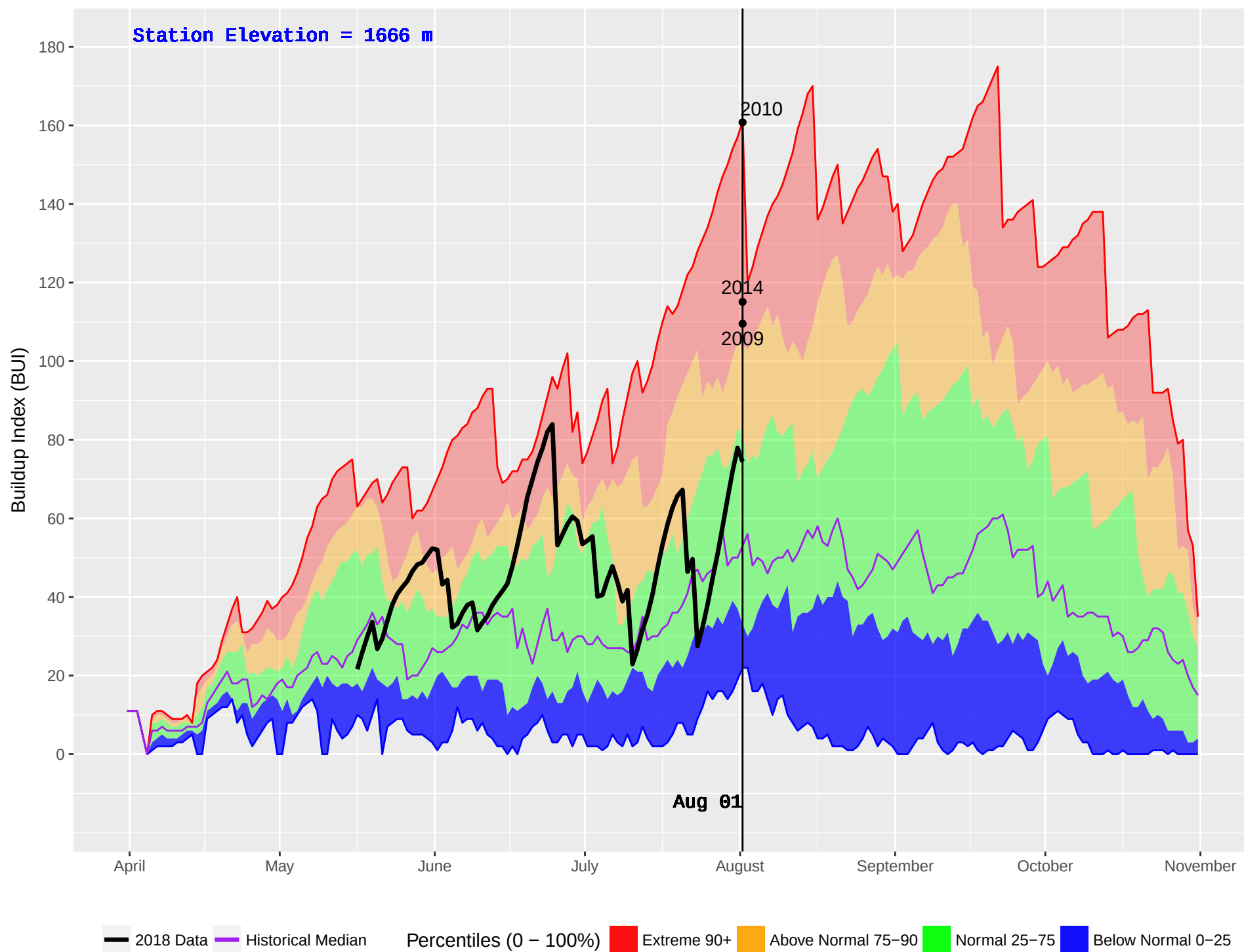
BALDFACE (221) : Historical (1992–2016) and Current (2018) Daily Buildup Index (BUI)
